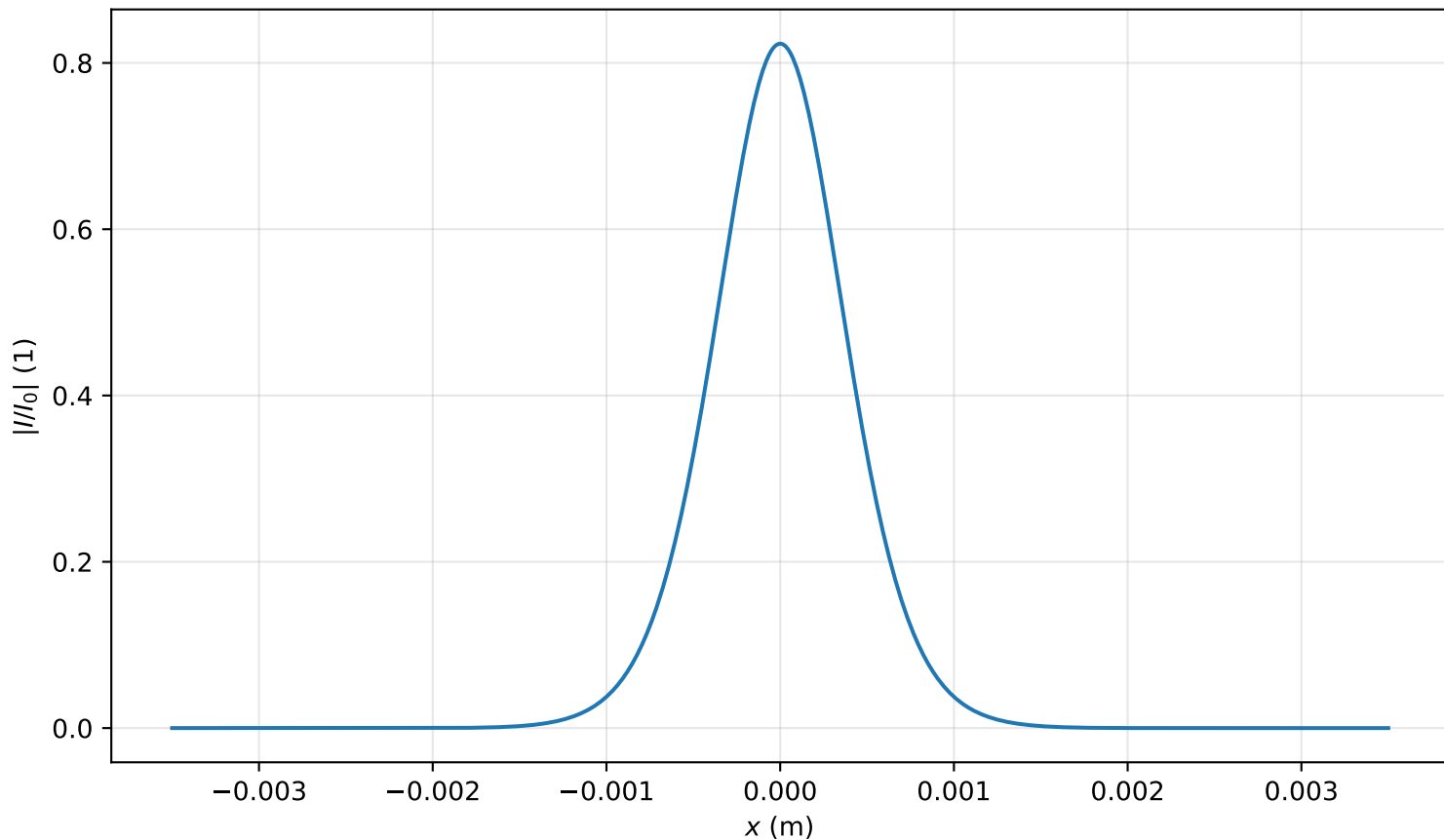
Intensity profile I(x, y = 0, z = 1.672m)/I_0 , P_{in}=0.4P_{cr} , artificial time
